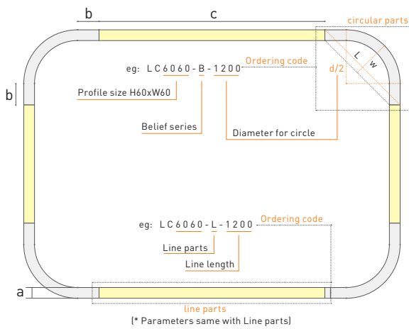
Case 1: if the diameter < 1.5m; b = 200mm
