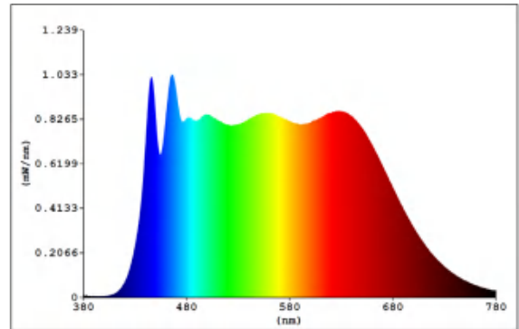
*@4000K, CRI>95, lower blue wave power
