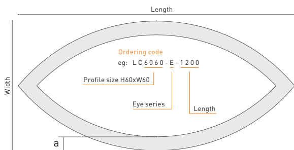
Case 1: if the length < 1.5m, profile is only 1 part
