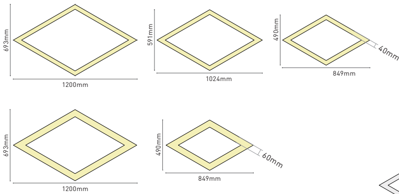
Case 1: if the length < 1.5m, profile & PC cover is only 1 part.
