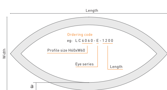
Case 1: if the length < 1.5m, profile is only 1 part
